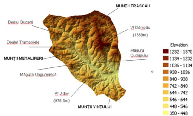
Fig. 2 The hypsometric map
